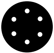
6" 6 VAC HOLES
